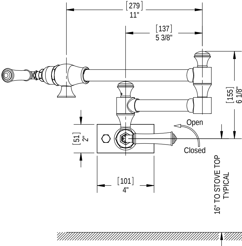
Critical Dimensions
