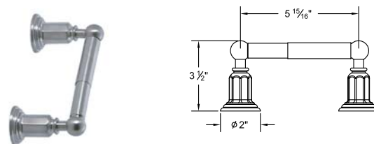
2965VA __ Paper Holder with Spring-Loaded Bar
