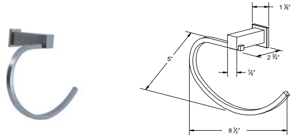
2864EM __ Towel Ring
