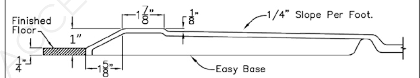
Detail of 1" Threshold
