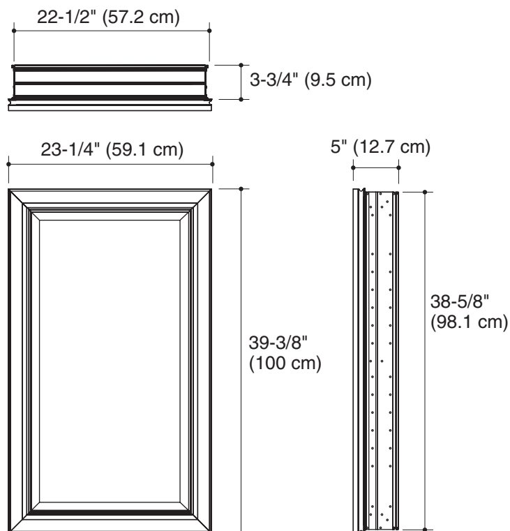
Product Diagram
