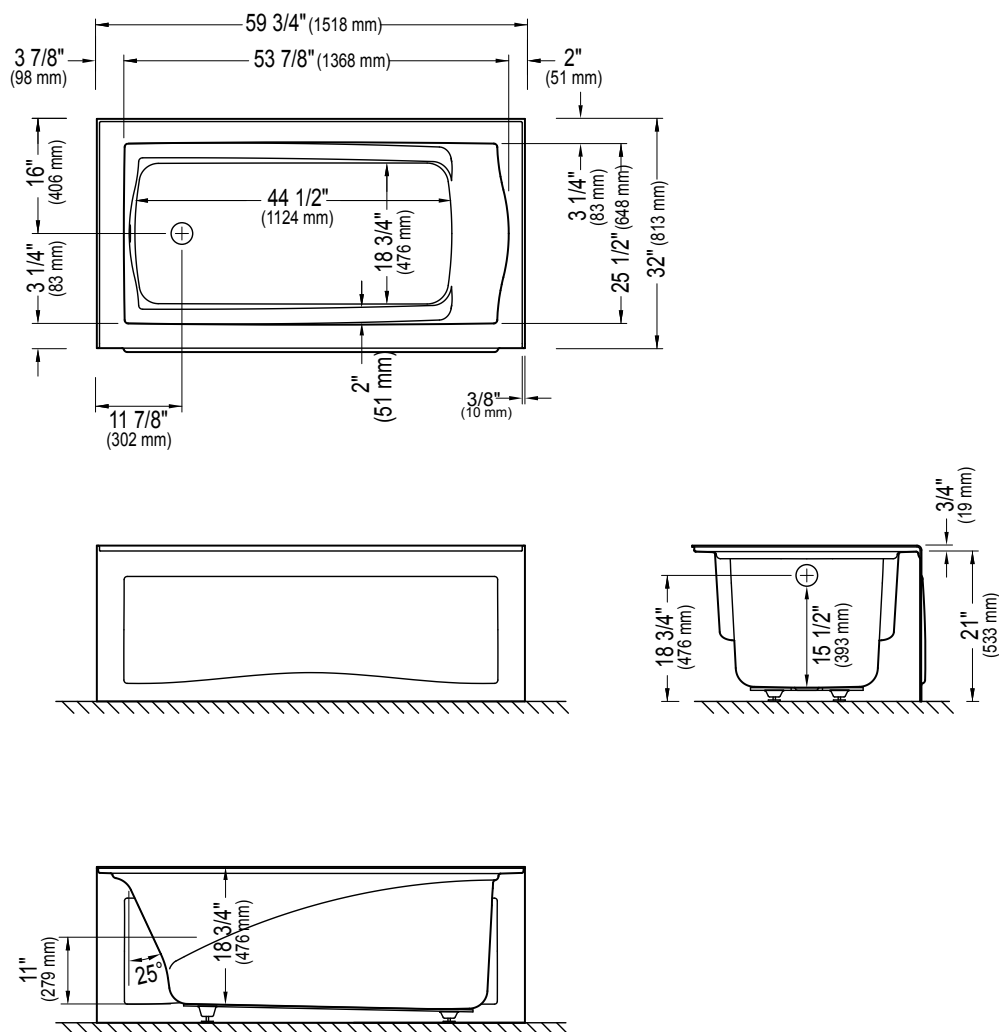
Rear view
