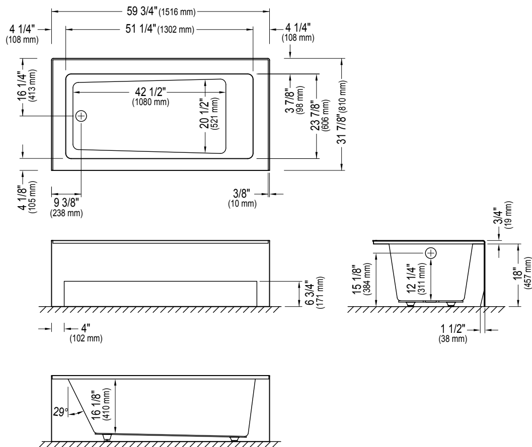
Rear view
